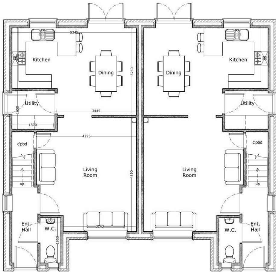
Proposed Ground Floor Plans
