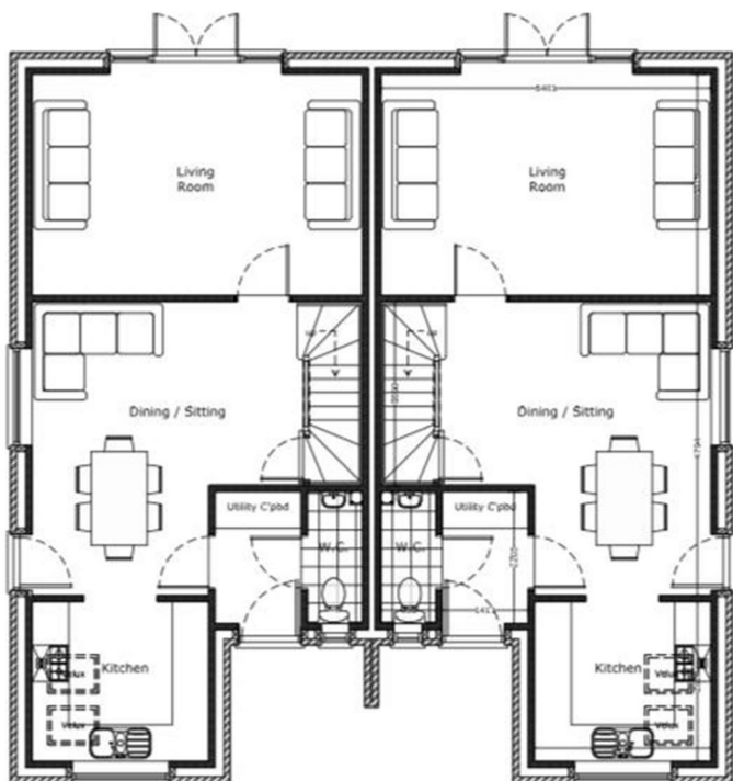
Proposed Ground Floor Plans Plots 27 - 30
