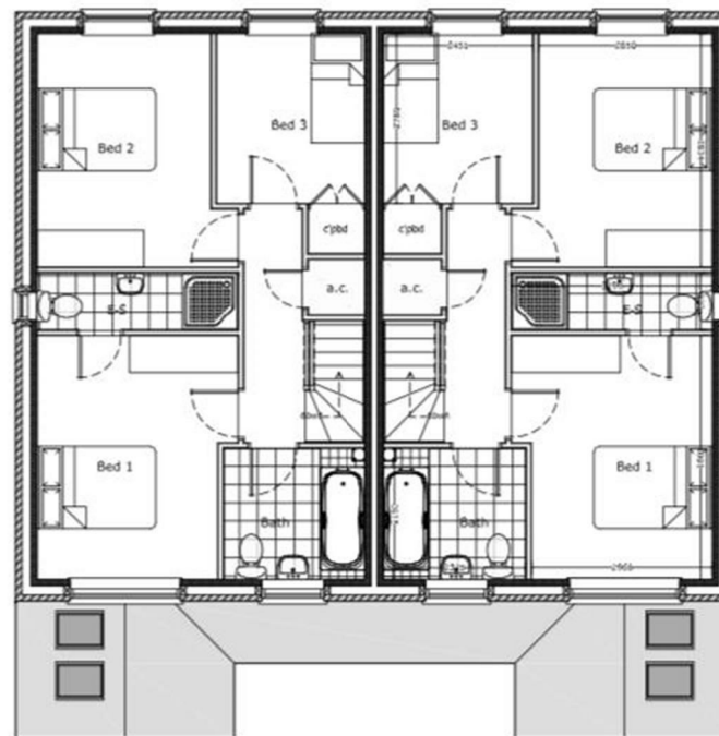
Proposed First Floor Plans Plots 27 - 30
