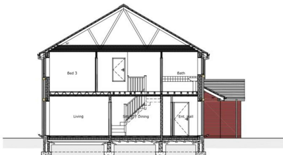
Proposed Section Through
