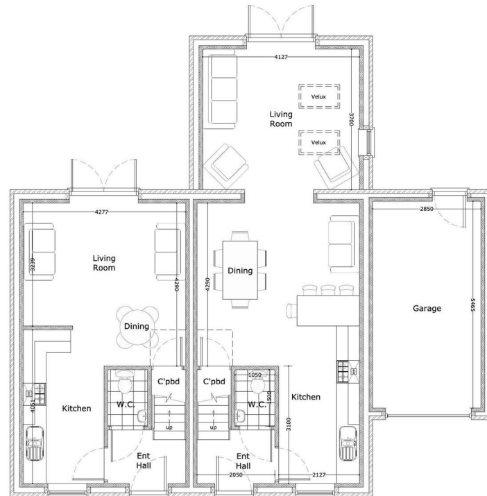
Proposed Ground Floor Plans
