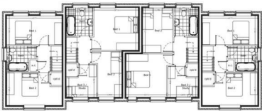
Proposed First Floor Plans
