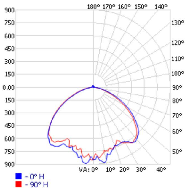
Polar Candela
