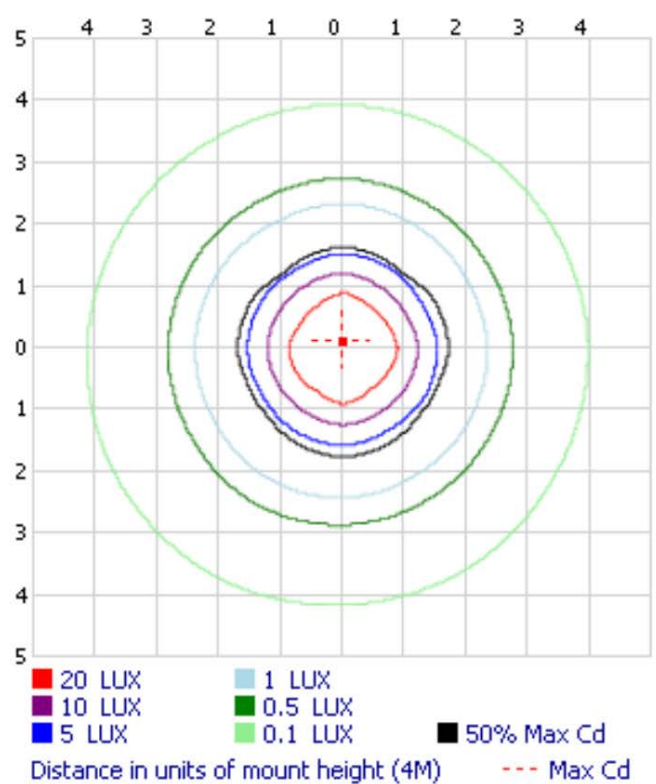
Isoilluminance
