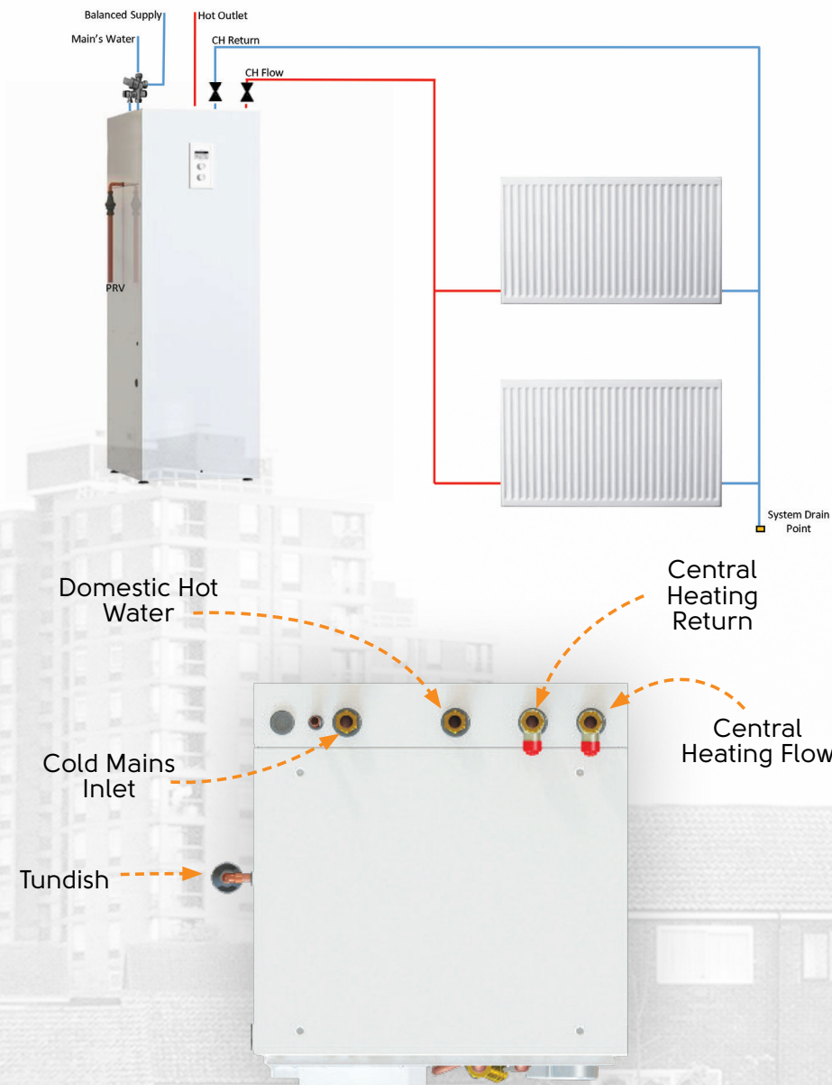
Top Entry Plumbing Connections
